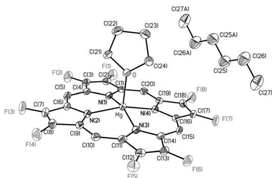
Figure 3. ORTEP drawing (50% thermal ellipsoid) of MgOFP with hydrogen atoms eliminated for clarity.
